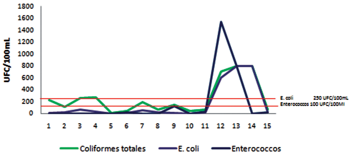
Figure 2. Concentration of pathogenic microorganisms in the water ballast tanks of vessels entering the Gulf of Morrosquillo, where 1. Alex spirit1 wbp, 2. Alex spirit 4 wbs, 3. NS columbus4nc, 4. NS columbus5nc, 5. Golf loast 4wbt, 6. Golf loast 4swbt, 7. Eric spirit swbp, 8. Eric spirit wbs, 9. Enrica lexle 4wbtp, 10. 3wbp, 11. 2wbs, 12. Kayeema spirit 4sw, 13 Kayeema spirit 3ew, 14 Chentrans lyra 4pw, 15. Chentrans lyra 4 sw. The green line is Total Coliform ; the blue is Enterococci , the purple, Escherichia coli .
