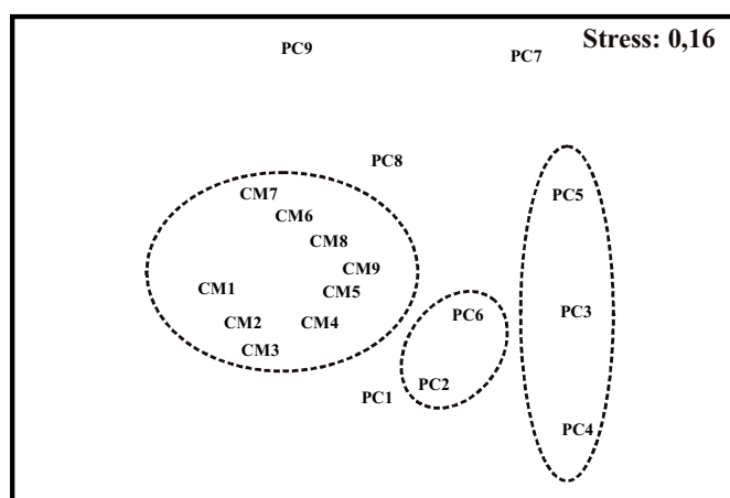
Figure 5. Analysis of classification and organization of the phytoplankton community in Cabo Marzo and Punta Cruces. The symbols represent the significance of the identified aggregations (routine SIMPROF, p < 0.05 ). CM: Cabo Marzo, PC: Punta Cruces. The number identifies the station in each location.
