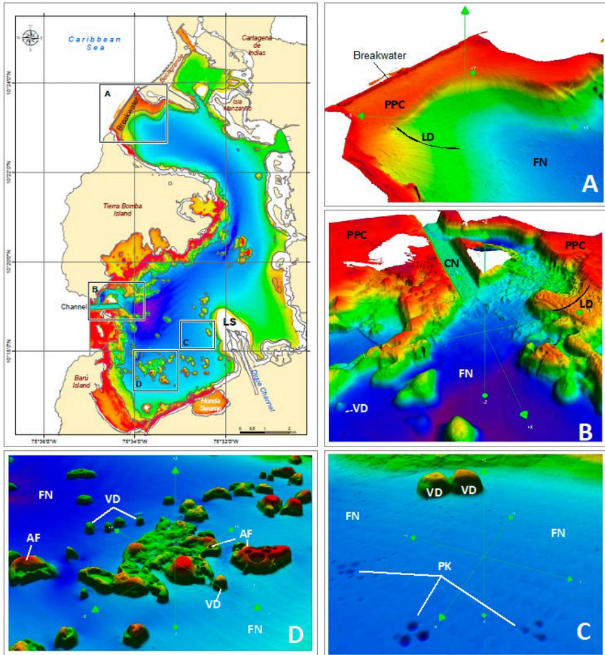
Figure 2. Geomorphological units: PPC: Continental shelf flat; LD: Slope; FN: Bay bottom; AF: Reef, VD: Mud volcano; PK: Pockmarks; CN: Channel; LS: Sediment fan; EC: Breakwater.
