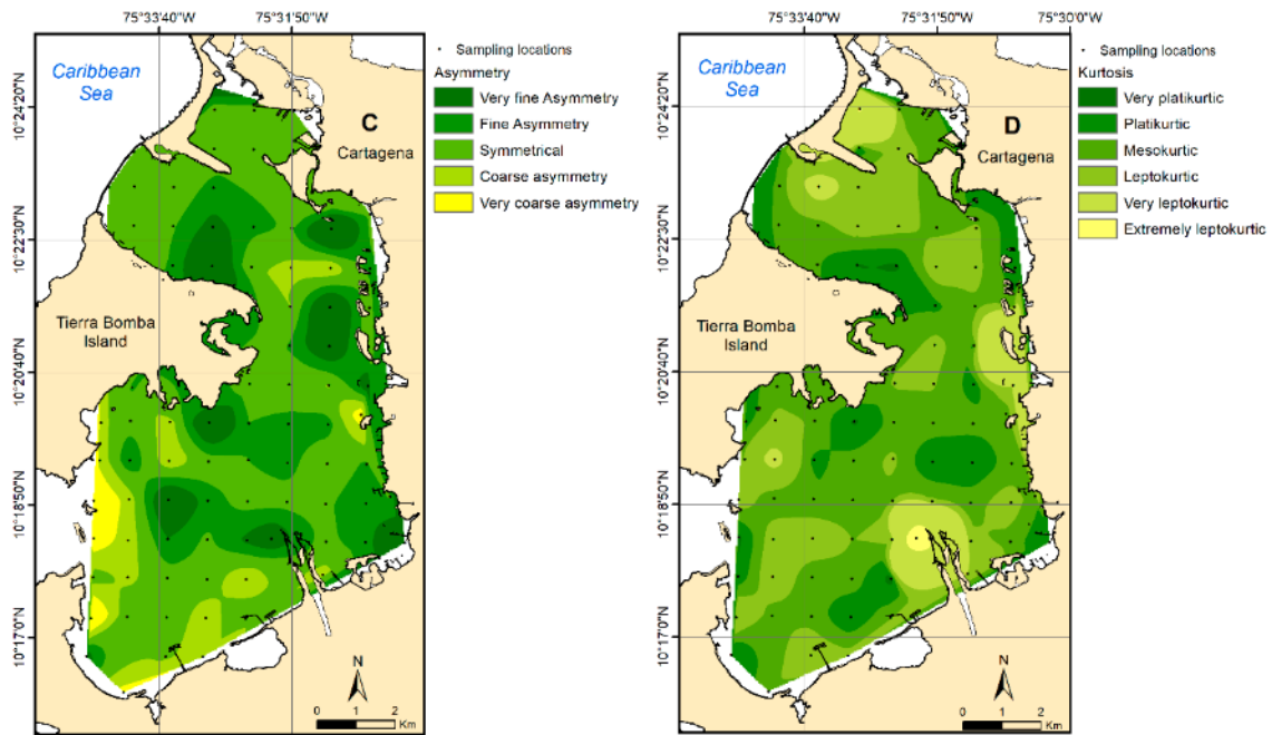
Figure 5. Visualization of the distribution of the texture characteristics of the surface sediments in Cartagena Bay.
