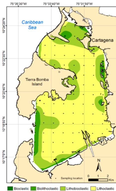
Figure 6. Visualization of the distribution of the composition of the surface sediments of Cartagena Bay.
