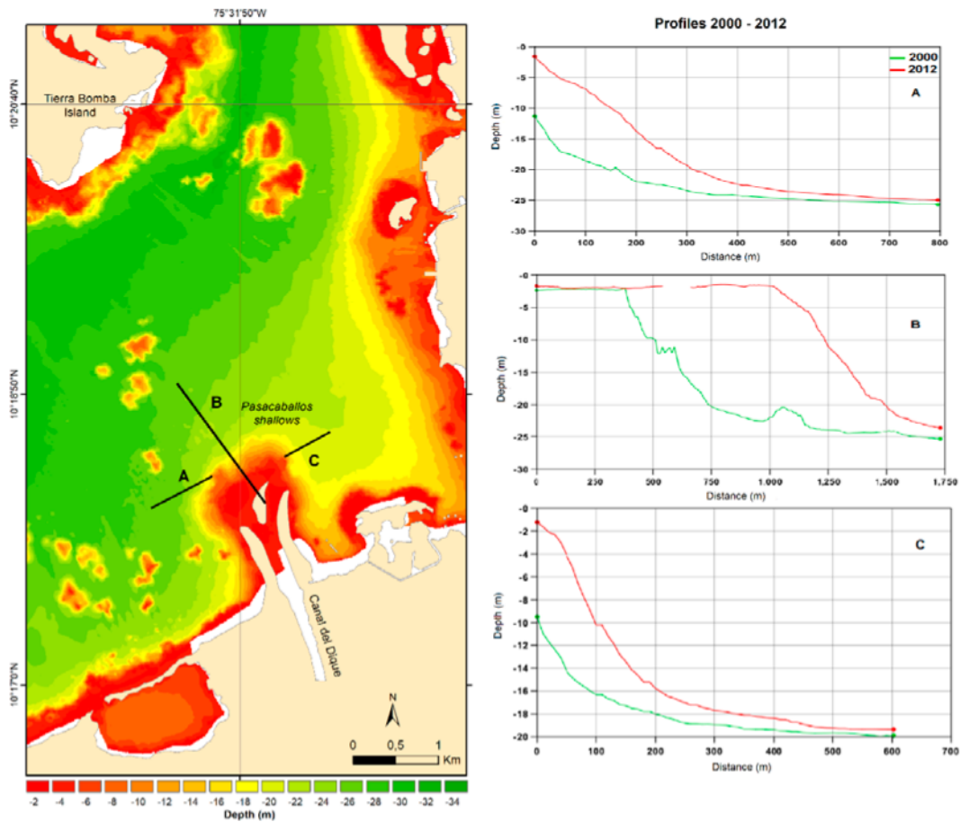
Figure 4. Depth profiles from the bathymetries for the years 2000 and 2012.
