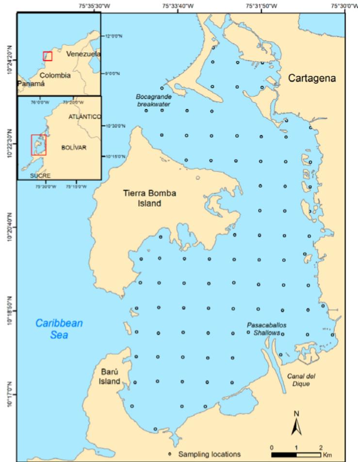
Figure 1. Location of the study area and sampling points (black dots).
