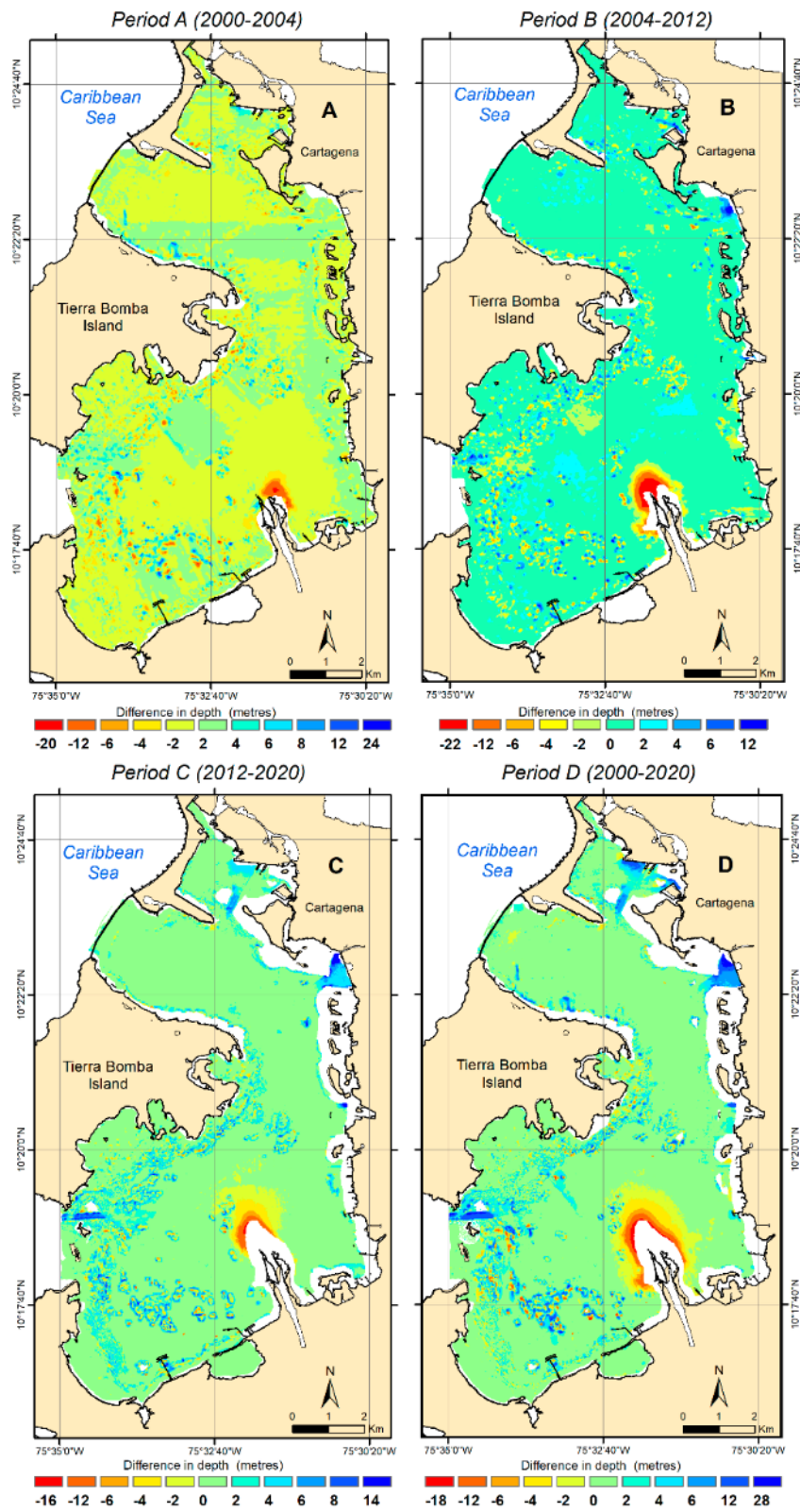
Figure 3. 2D view of the difference between the bathymetries of Cartagena Bay in four periods during the last 20 years
