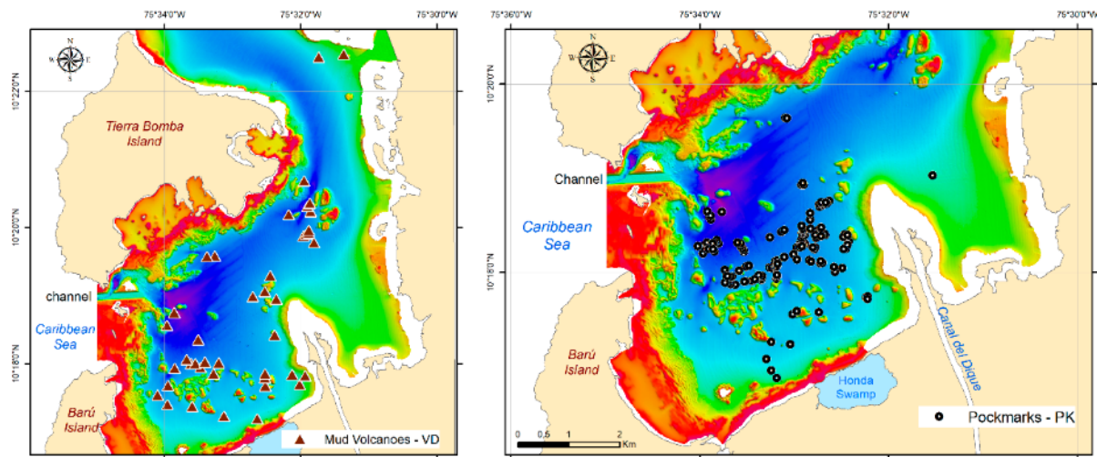
Figure 7. Location of Mud Volcanoes (VD) and Pockmarks (PK) in Cartagena Bay.
