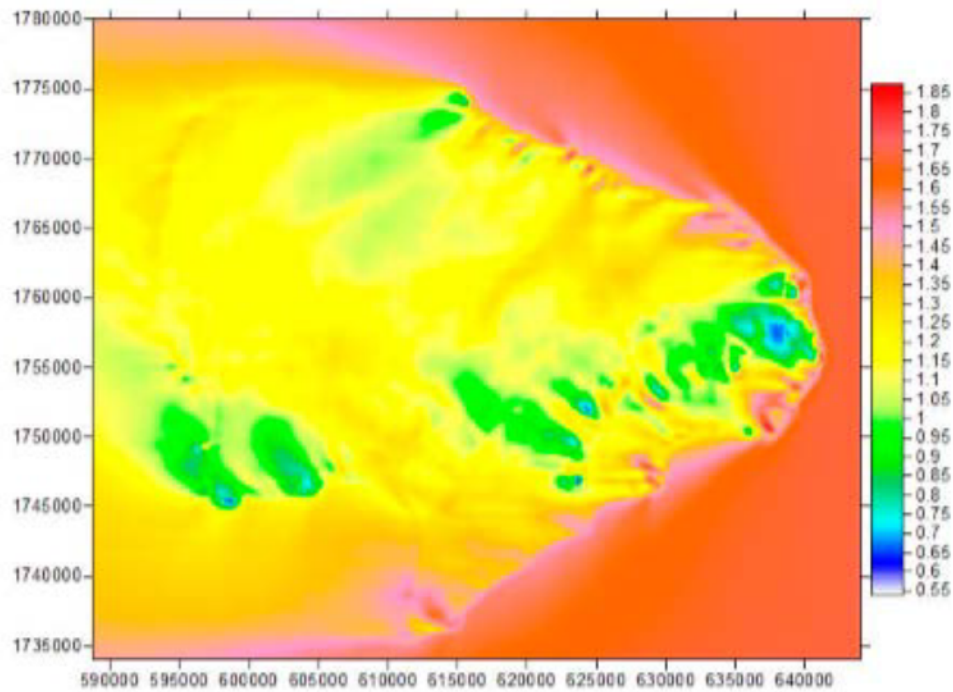
Figure 9. Wave propagation (significant height in meters) for the extended domain under the dominant weather conditions, analyzed with data from the WW-III model. Outputs of the SWAN model.
