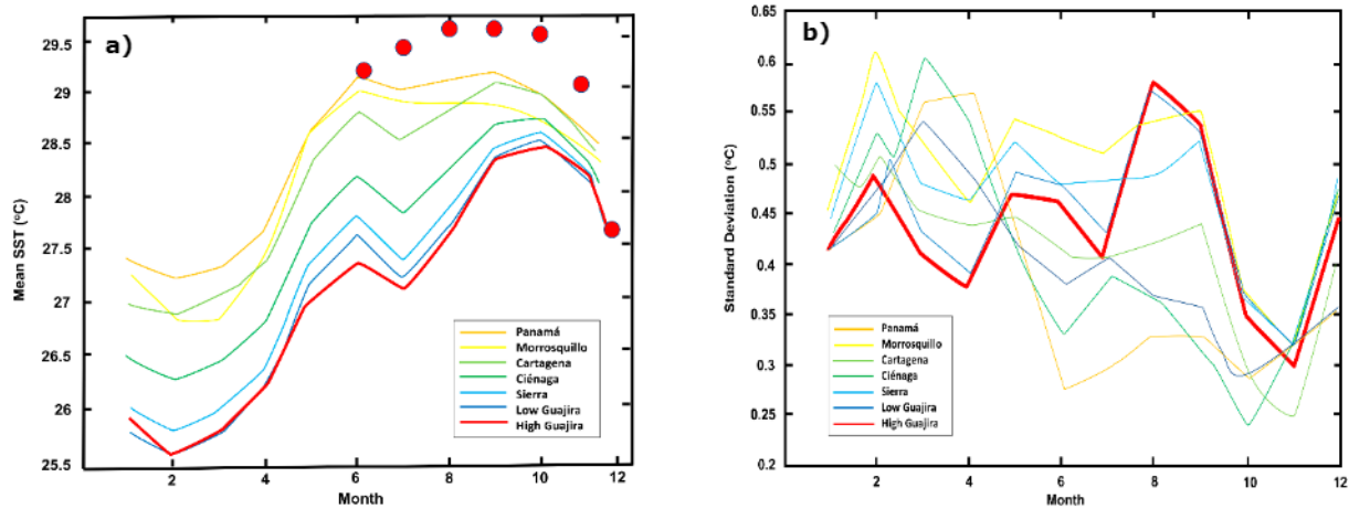
Figure 5. SST (a) and standard deviation in SST figures (b) presented in Bernal et al. , 2006 (continuous lines) and found in this work during the second half of 2020 (red dots).
